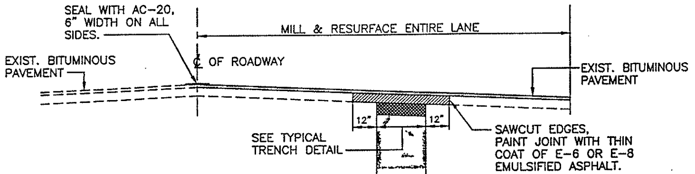
SECTION B-B
