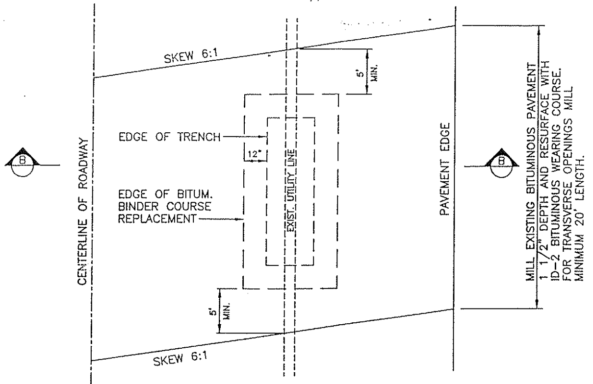
PLAN - PAVEMENT RESTORATION DETAIL 'B'
